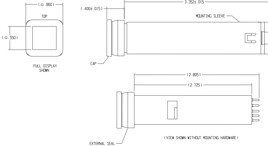
SWITCH ASSEMBLY
